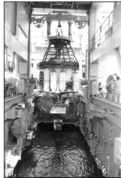
Figure 1-20. PTC Handling System, Elk River .
